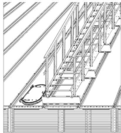
— Dwg of roof stairs front view
