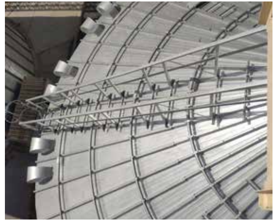
— Photo of roof ladder with front landing
